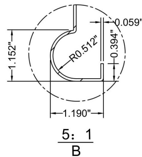
Mixing Valve
